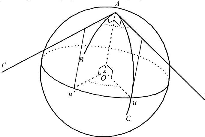
FIG 9 : \widehat{A} = \widehat{tAt'} = \widehat{uOu'}
