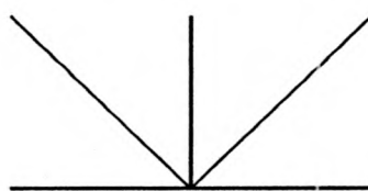
allure de f_i , c_i = 0
