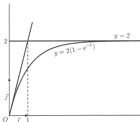
a) E = 2 \quad \tau = 1
